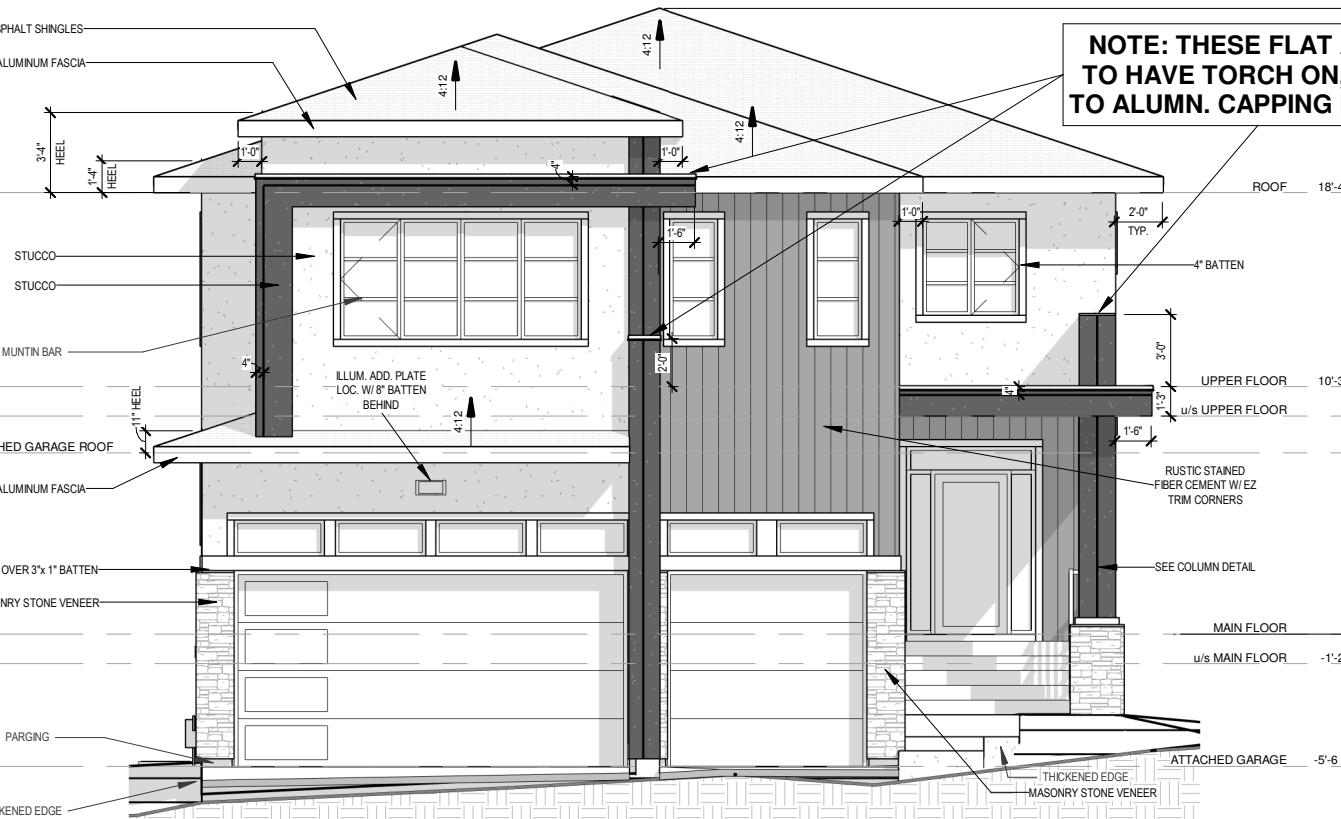
FRONT ELEVATION 1/8" = 1'-0"
